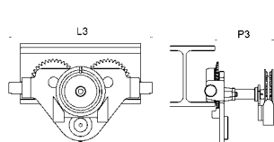
Model HTG 500 - 5000 kg with rotating hand chain guide and buffers
